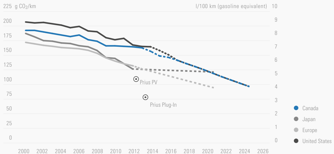
Figure 26 Historical Fleet CO 2 Emissions Performance and Proposed Standards for Cars
