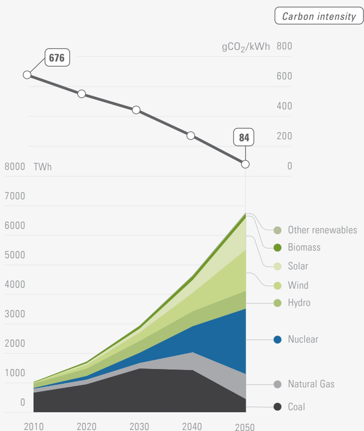
Figure 6. Energy Supply Pathway for Electricity Generation, by Source
