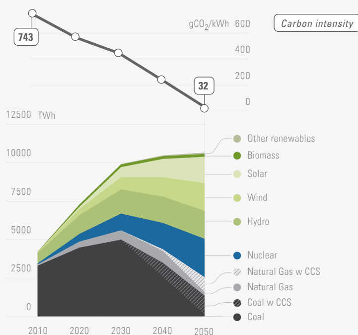
Figure 6. Energy Supply Pathway for Electricity Generation, by Source
