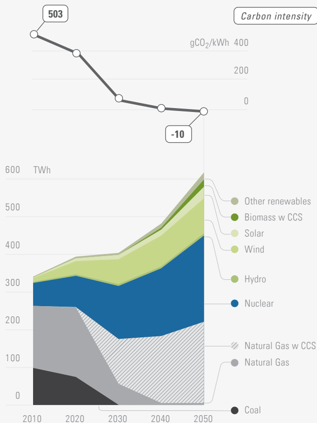
Figure 6. Energy Supply Pathway for Electricity Generation, by Source
